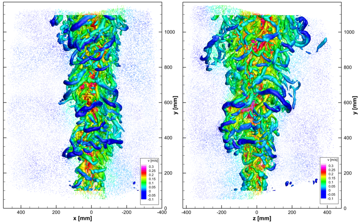
Figure 11: Isosurfaces of Q-criterion for one time-instant, color-coded by streamwise velocity. (Left) front view (looking from the cameras); (right) side view. Isosurfaces superimposed on the tracks as shown in Figure 10
