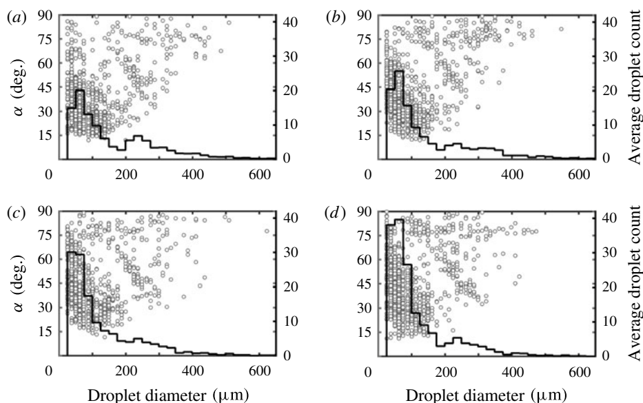
FIGURE 18. Ensemble averaged size distributions of airborne droplets per realization (12–25 experiments) for (a) the control case, (b) oil with h = 30\ \mu\text{m} , (c) oil with h = 400\ \mu\text{m} and (d) an h = 500\ \mu\text{m} layer of dispersant–oil mixture with DOR = 1:25. The minimum resolution is 12.4\ \mu\text{m} and the bin width is 24.9\ \mu\text{m} . Also shown are scatter plots of the corresponding droplet elevation angle \alpha for 10 realizations for each of the four cases. The bottom of the field of view in which these data are acquired is located at y = 13\ \text{mm} .
