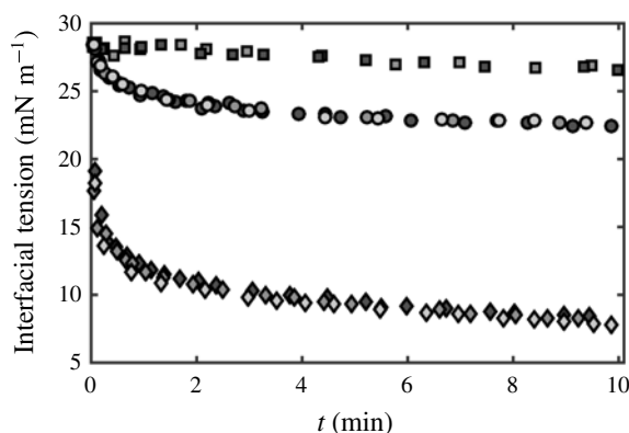
FIGURE 23. Dynamic surface tensions of crude oil (squares) and premixed dispersant–oil mixture with DOR 1:25 (circles) at 22 °C. Dynamic interfacial tension of crude oil with seawater (diamonds) at 19 °C. The measurements were performed with the pendant drop technique. Grey level shadings indicate replicate measurement series.
