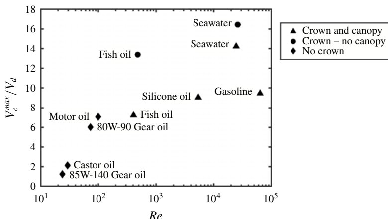
FIGURE 11. Cavity volume at maximum cavity depth ( V_c^{\max}/V_d ) as a function of Re for droplet impact on thick oil layers ( h = 5.7d ) and for droplet impact on water (both for d = 3.8 mm, u = 7.28 m s ^{-1} ). The symbols indicate crown behaviour and correspond to the same symbols as in figure 10.
