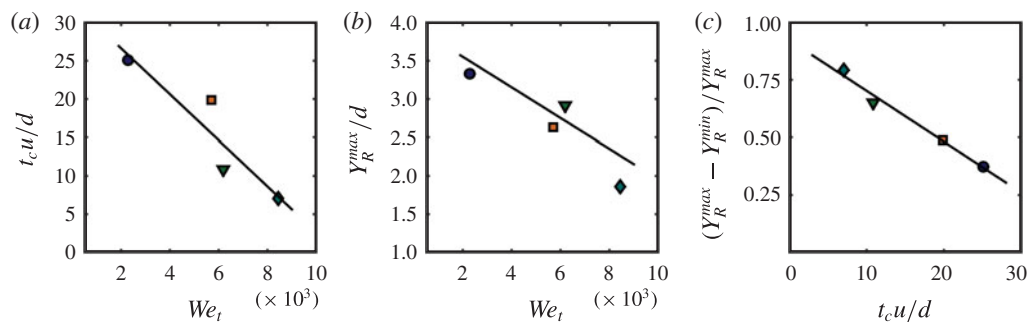
FIGURE 13. (Colour online) (a) Bubble canopy closure time t_c u/d as a function of We_t . (b) Maximum height of crown Y_R^{max}/d as a function of We_t . (c) Canopy ceiling fall distance (Y_R^{max} - Y_R^{min})/Y_R^{max} as a function of canopy closure time t_c u/d . The symbols correspond to the fluid types in figure 12.
