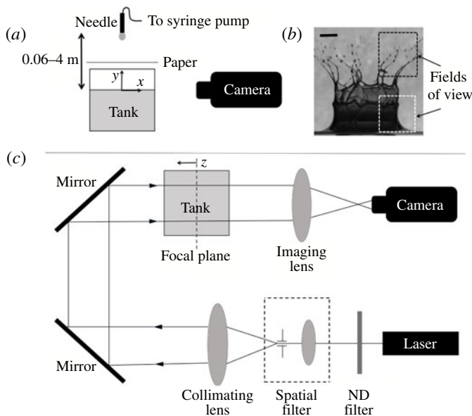
FIGURE 2. (a) Set-up for high-speed visualization experiments. (b) A sample image showing the fields of view of holographic observations relative to the splash crown and liquid surface ( t = 3 ms after impact; h = 400 \mu\text{m} ). The upper field of view (black outline) is used for measuring droplet statistics while the lower field of view (white outline) is used for examination of droplet generation mechanisms at early time points. The scale bar is 4 mm. (c) Top view of the holographic set-up.
