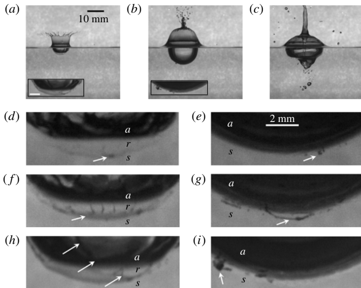
FIGURE 5. (a–c) Sample images showing the impact of the water droplet (same as in figure 3) on an oil layer of thickness h = 100\ \mu\text{m} . The insets (all at the same magnification) show magnified sections of the images. The white inset scale bar at 1 ms in (a) is 2 mm: (a) 1 ms, (b) 8 ms and (c) 43 ms. (d–i) Magnified images showing the oil layer rupture and breakup for oil layer thicknesses of (d,e) h = 10\ \mu\text{m} , (f,g) h = 30\ \mu\text{m} and (h,i) h = 100\ \mu\text{m} . Here, a is the air cavity, r is the raindrop fluid layer and s is the seawater. The arrows show the retracting oil film at 1 ms (d,f,h) and the collected oil droplets at 8 ms (e,g,i).
